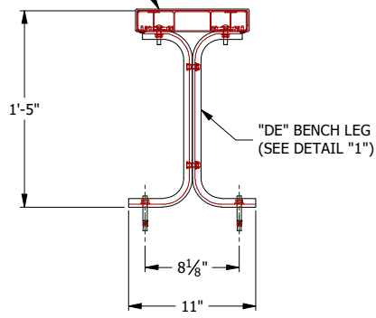
CONCRETE ANCHORED OPTION SEE DETAIL "3"
