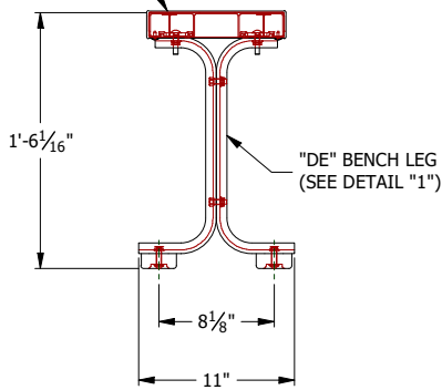
RUBBER FOOT PAD OPTION SEE DETAIL "2"
